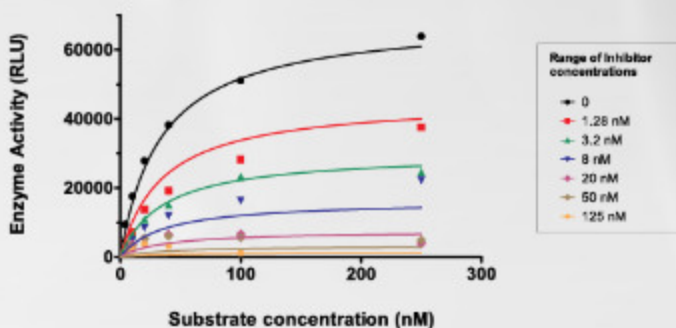
Figure 2: IC_{50} determination of a kinase
